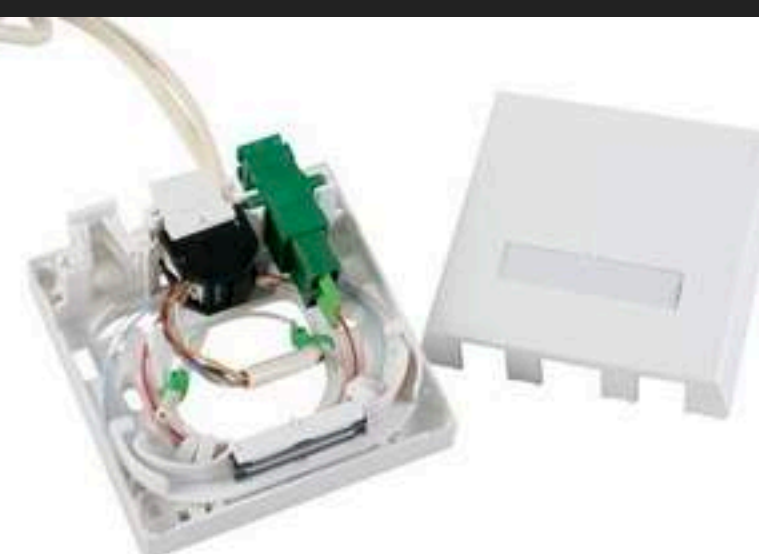
Wall outlet FTTH
